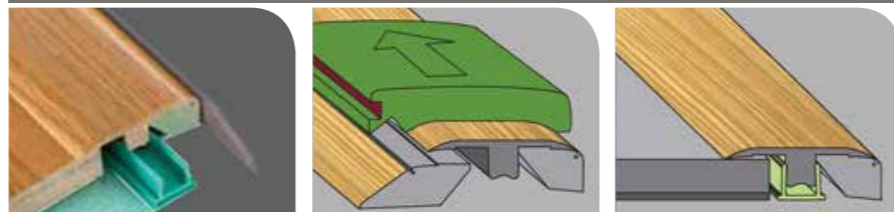
ENDPROFIL. THRESHOLD. PERFIL FINAL.
